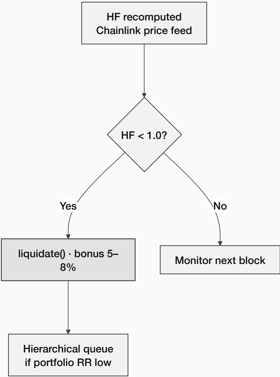
(a) LiquidationEngine
