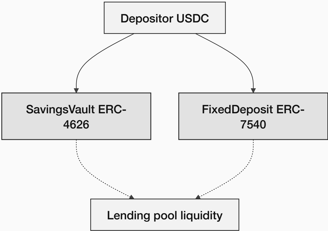
(b) SavingsVault · FixedDeposit
